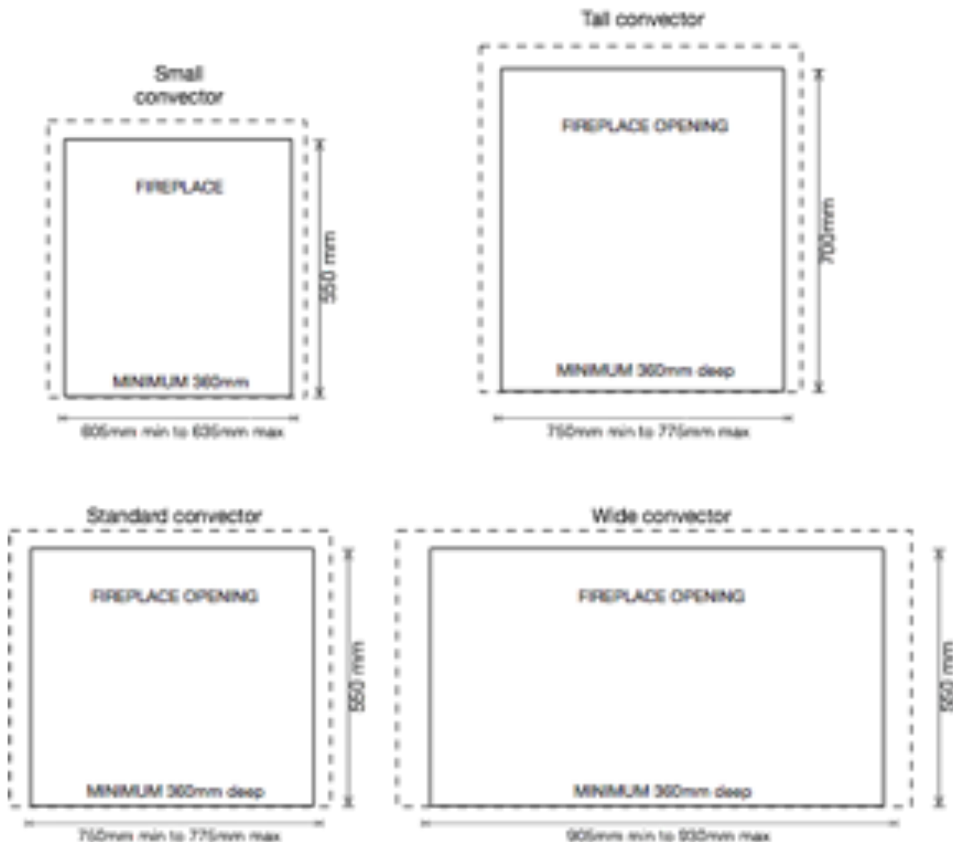
Fireplace opening sizes and catchment space
